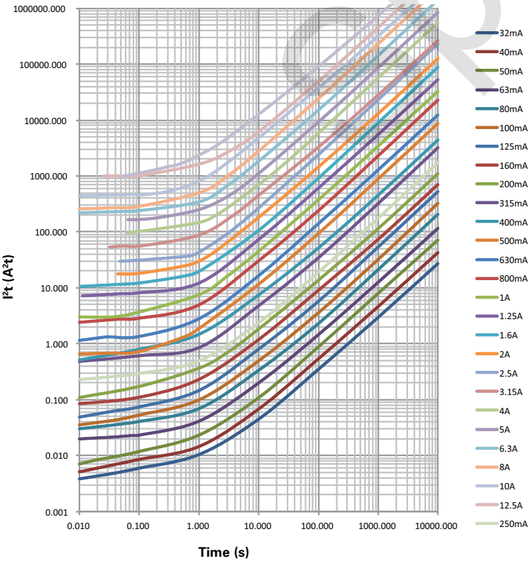
I^2t vs. time curve
